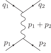
Fig. 10.1. The three-level Feynman diagram for the scattering \mu^-(p_1) + \mu^+(p_2) \rightarrow e^-(q_1) + e^+(q_2)
